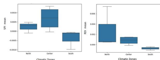
Figure 7. Distribution of SPI-mean and RDI-mean Across Climatic Zones (North, Center, and South).
