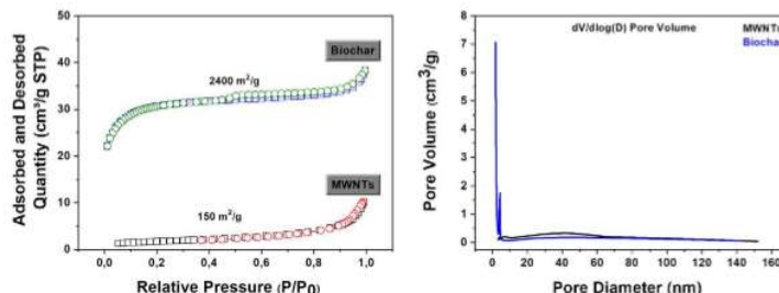
Fig. 6: N 2 adsorption–desorption isotherms (left) and their corresponding pore size distributions (right).
