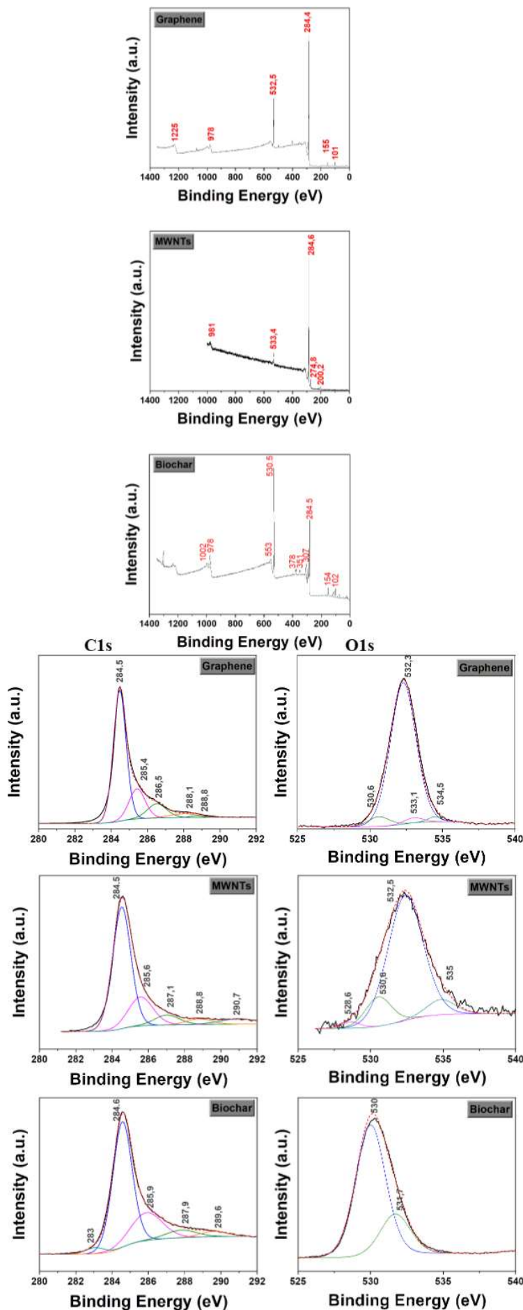
Fig. 7: Expanded XPS survey spectra and their deconvoluted C1s and O1s for graphene, MWNTs and biochar.
