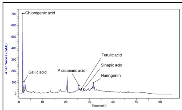
Fig B. HPLC chromatograms of O.ficus-indica seed extracts (Extract Ethanol 40%) at 280 nm [22].
