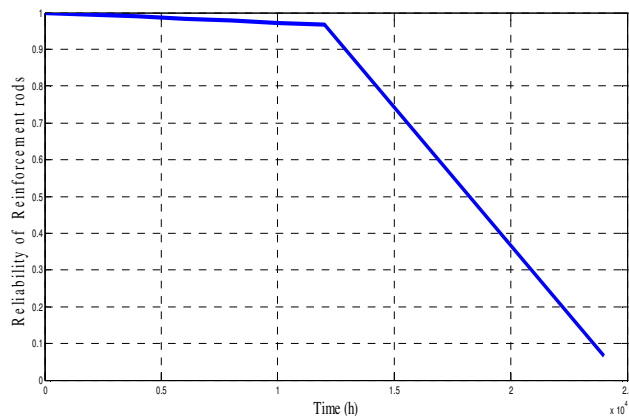
Fig. 7: Reinforcement rods
