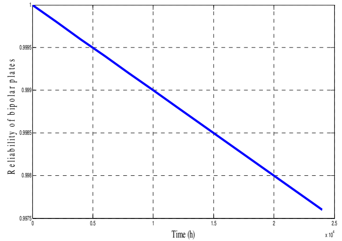
Fig. 5: Bipolar plates
