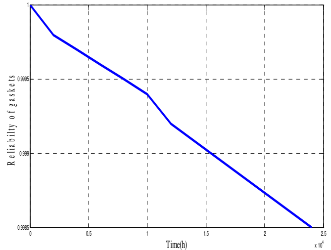
Fig. 6: Gaskets
