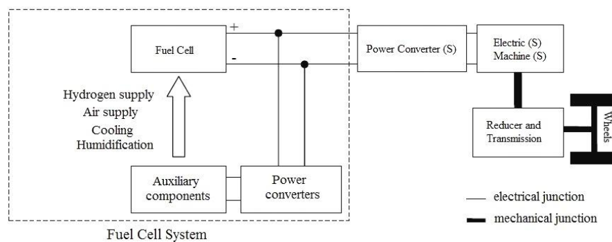
Figure 13: Example of Fuel Cell Power train Architecture.
