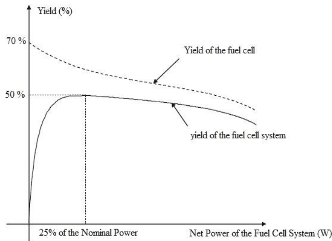
Figure 12: Characteristics yield of the fuel cell and fuel cell system.
