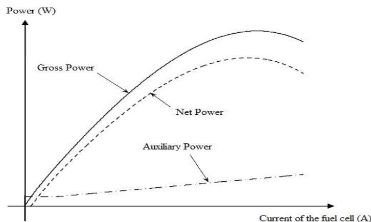
Figure 11: Characteristic powers of a fuel cell system (gross, net and auxiliary power).
