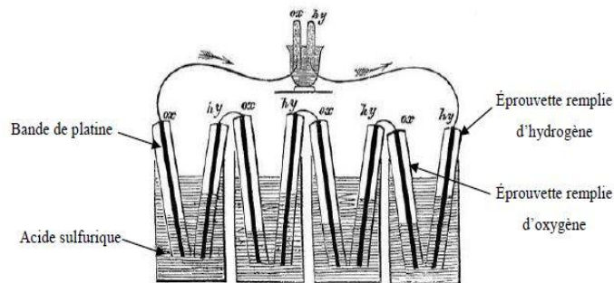
Figure 3: The Sir William Grove experience
