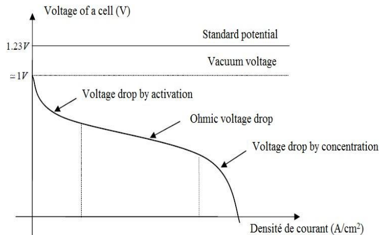
Figure 9: Conventional polarization curve of a PEM fuel cell.
