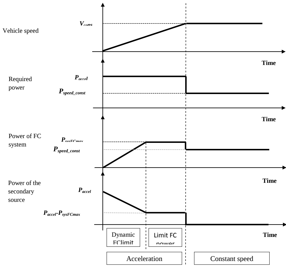
Figure 16: Example of the powers involved in accelerating and maintaining the speed of the vehicle.
