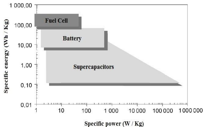
Figure 15: Plan of Ragone[40].
