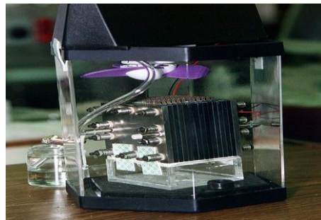
Figure 4: Fuel Cell, from NASA to Methanol[13].
