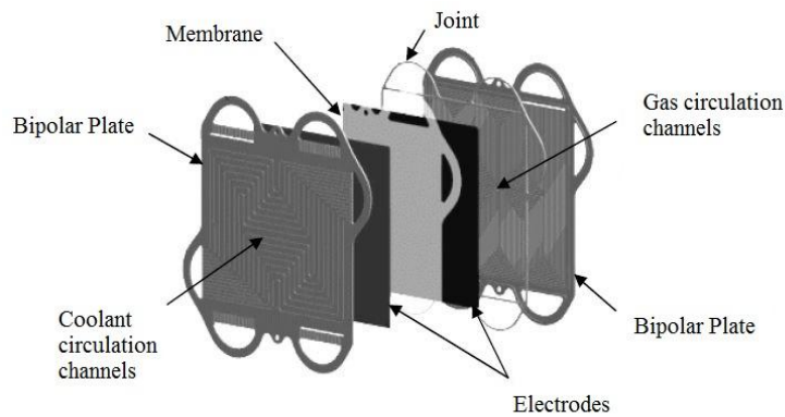
Figure 7: Example of assembly of an elementary cell [19]
