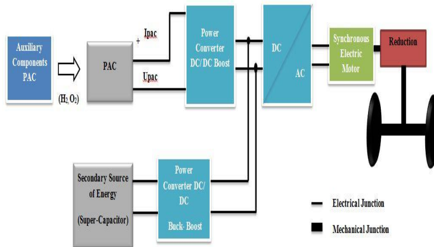
Figure 14: Example for Hybrid Fuel Cell Vehicle Architecture
