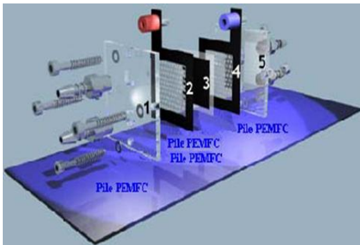
Fig.2 Single cell of H-Tec pemfc Cder.
