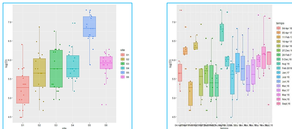
Fig. 10. Evolution of chlorides in time and space
