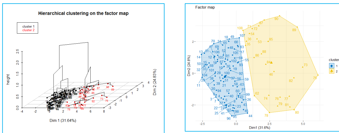
Fig.6. Hierarchical classification of individuals
