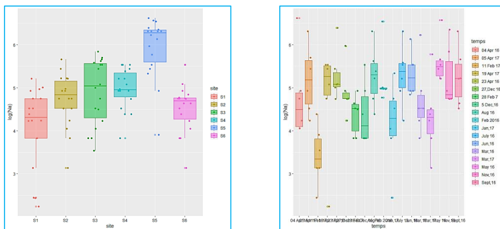
Fig.13. Evolution of sodium in time and space
