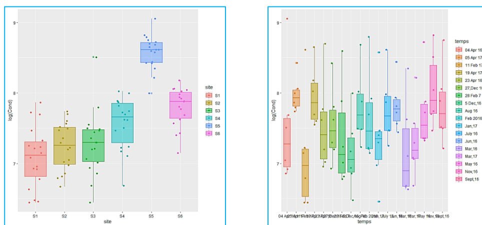
Fig.9. Evolution of conductivity in time and space
