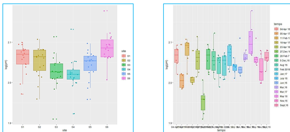
Fig.8. Evolution of pH over time and space
