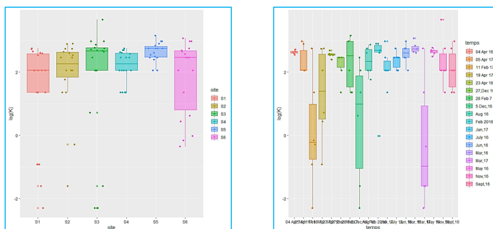
Fig.16. Evolution of potassium in time and space
