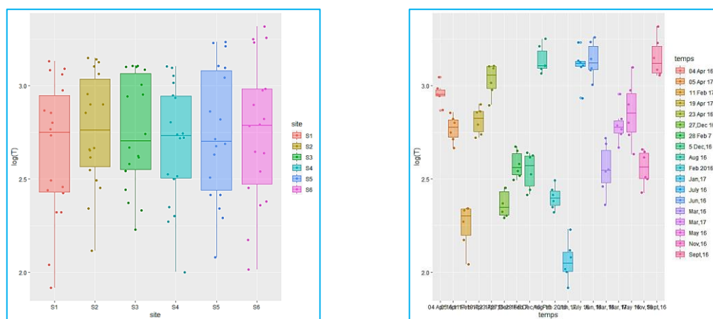
Fig. 7. Temperature evolution in time and space
