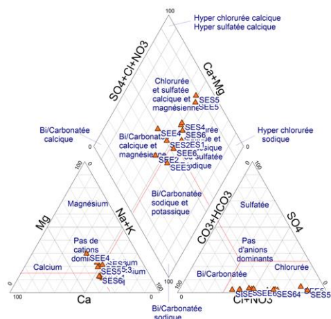
Fig.2. Piper diagram of purified water
