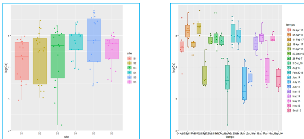
Fig.14. Evolution of calcium in time and space
