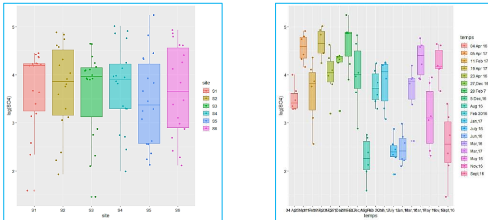
Fig.12. Evolution of sulphates in time and space
