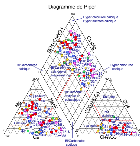
Fig.3. Piper diagram show hydrochemical facies according to hydrology
