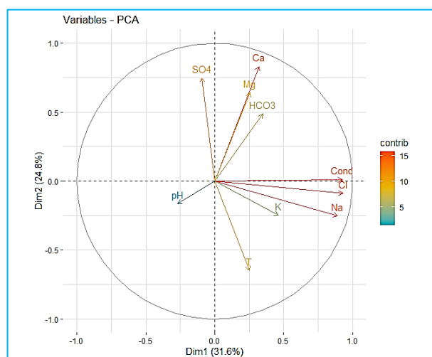
Fig.4. Correlation circle of physico-chemical variables
