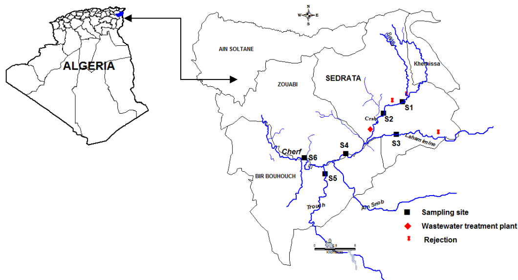
Fig.1. Map of location of sites and study area
