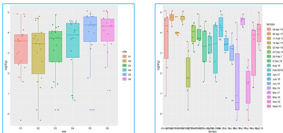
Fig. 15. Evolution of magnesium in time and space
