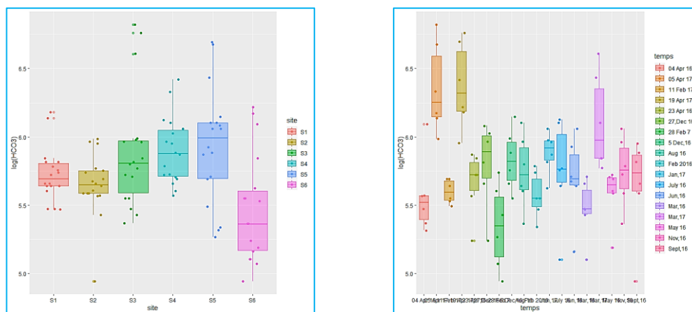
Fig. 11. Evolution of bicarbonates in time and space
