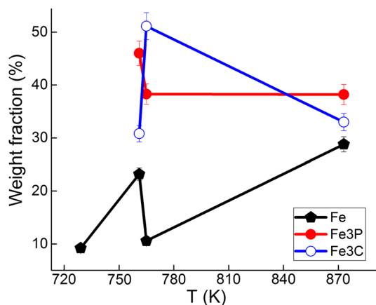
Fig. 5 Variation of the weight fractions of \alpha -Fe-type, \text{Fe}_3\text{P} -type and \text{Fe}_3\text{C} -type phases as a function of the annealing temperature
